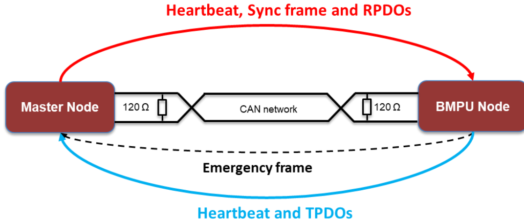
Figure 26: CAN network illustration
