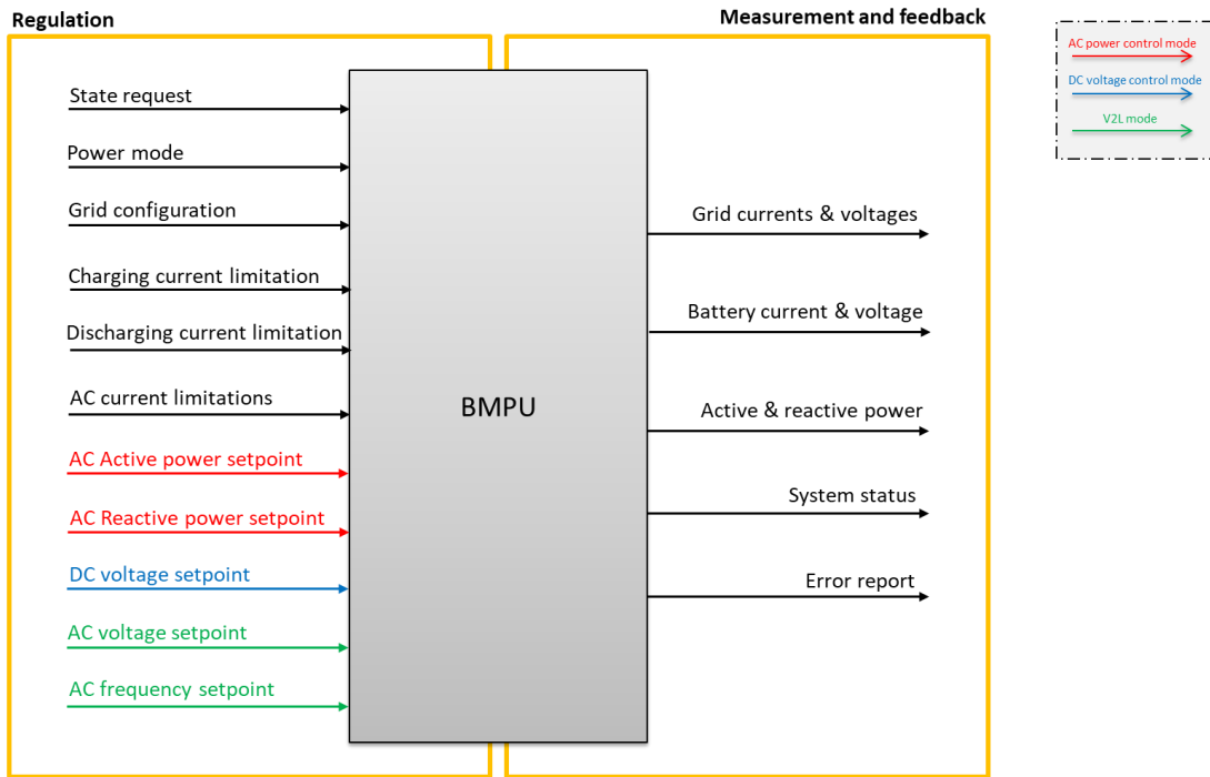
Figure 26: High level charger regulations and measurements
