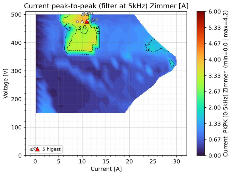
Figure 9: peak-to-peak current ripple at the battery side filtered at 5kHz given for grid conditions three-phase with neutral 400V/50Hz and SW version 2.5.4r (build 19020)
