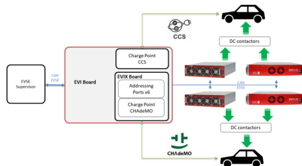
Figure 34: EVI & EVIX integration on EVSE environment
