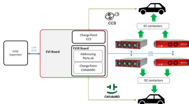
Figure 28: EVI & EVIX integration on EVSE environment
