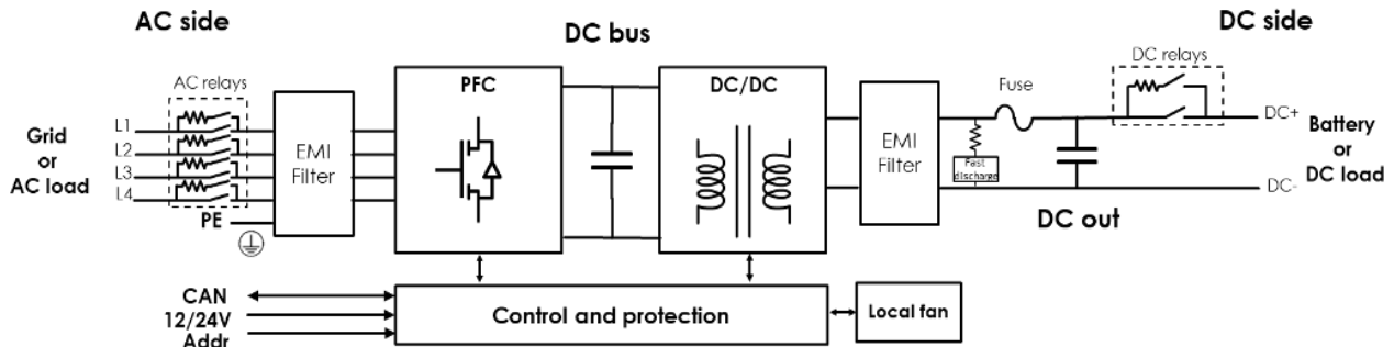
Figure 19 Converter synoptic
