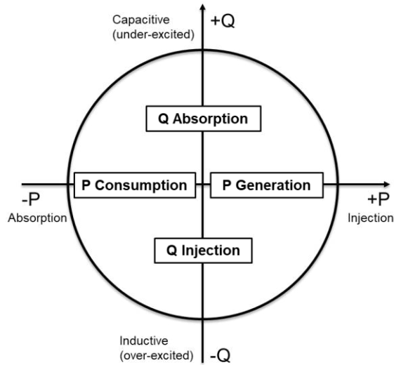
Figure 24: Power setpoint sign convention
