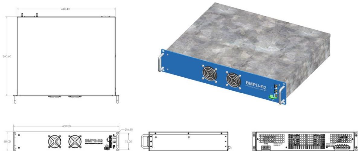
Figure 33: BMPU-R2 assembly drawing (with default real panel support)
