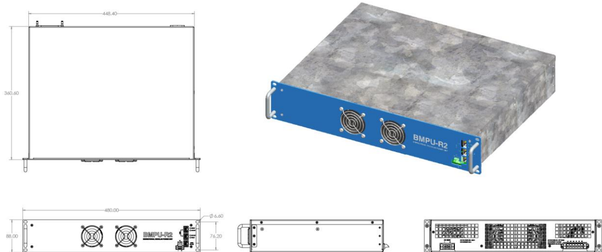
Figure 27: BMPU-R2 assembly drawing (with default real panel support)
