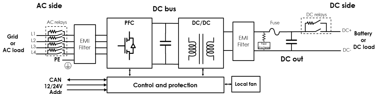
Figure 25 Converter synoptic
