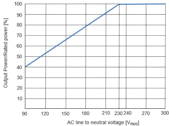
Figure 14: Output power vs AC line voltage (phase-neutral)
