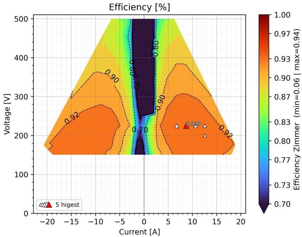
Figure 11: Typical BMPU-R2 efficiency in single-phase mode
