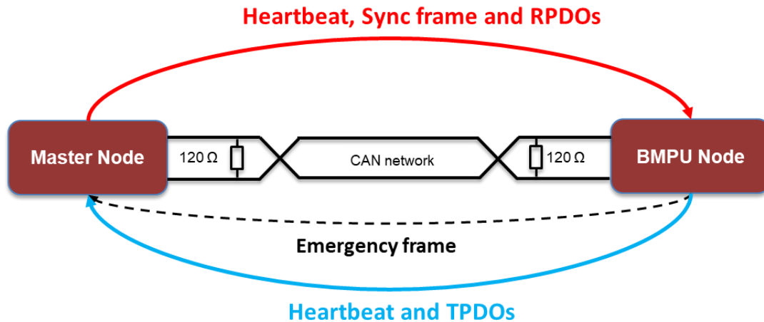
Figure 32: CAN network illustration
