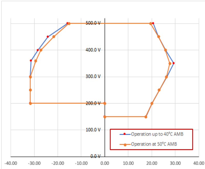
Figure 12: power derating at 50°C ambient
