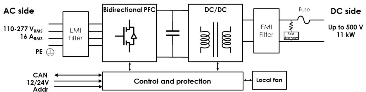
Figure 17 BMPU-R2 11 kW high level synoptic
