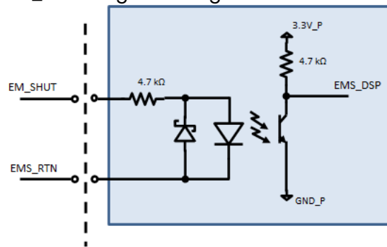
Figure 23 EMS input circuit
