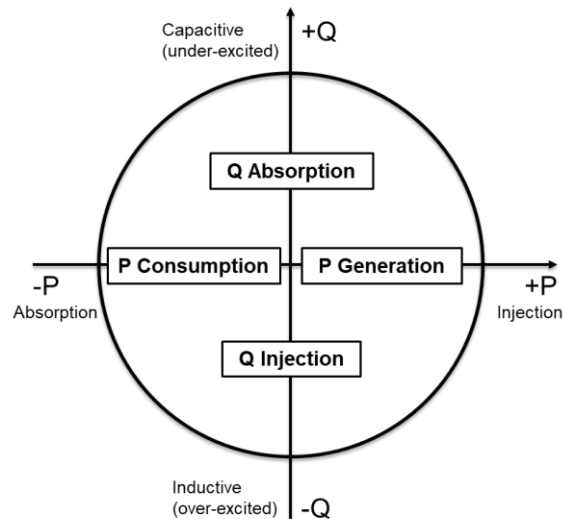
Figure 30: Power setpoint sign convention
