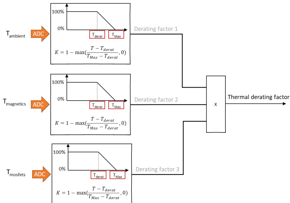
Figure 23 Thermal derating
